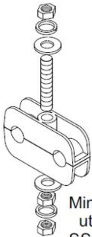
Mini Block Double Stack utilizing HK-DSCB or HK-DSCB158 Hardware Kit. (Mini Blocks ordered separately)
