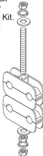
Mini Block Triple Stack utilizing HK-TSCB or HK-TSCB158 Hardware Kit. (Mini Blocks ordered separately)
